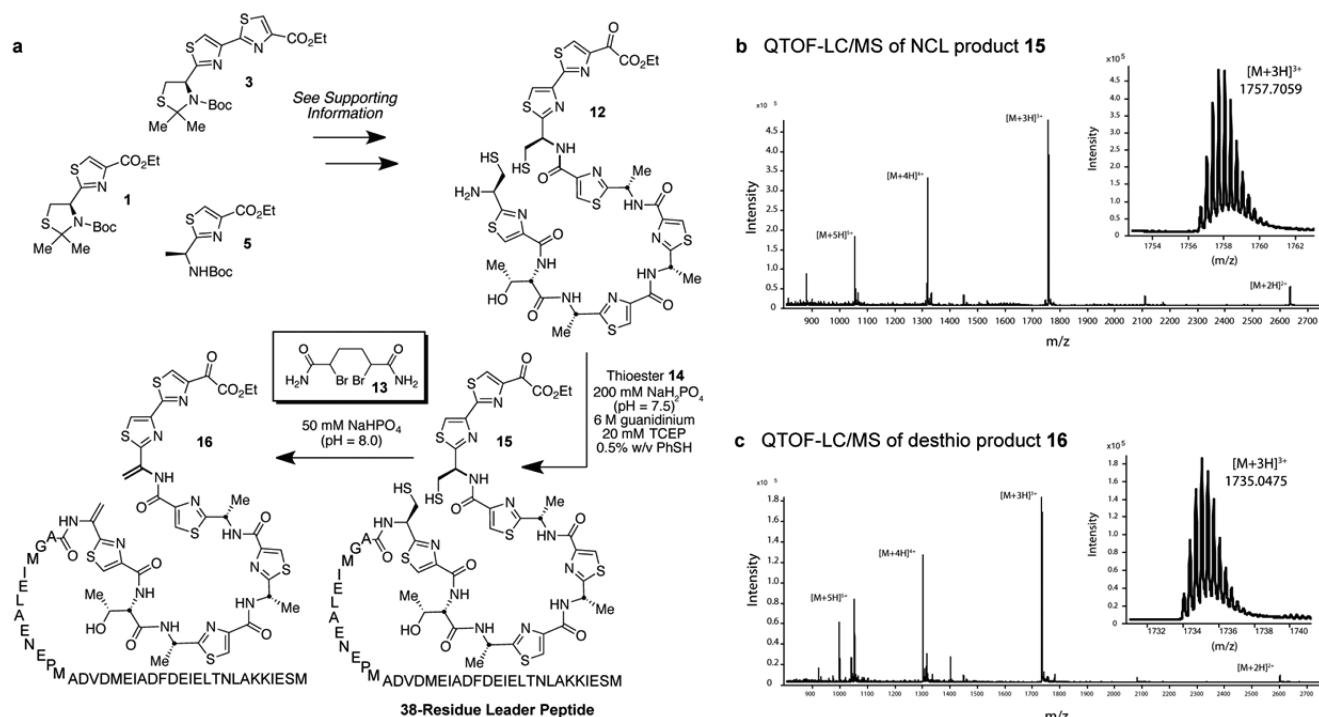
Figure 2. (a) Synthesis of the TcIM substrate by thiophenol-catalyzed native chemical ligation and sulfhydryl elimination with dibromoadipamide. (b, c) QTOF-MS data of (b) NCL product 15 and (c) elimination product 16 .
